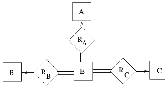
Figure 2.17 E-R diagram to Exercise 2.17b.
