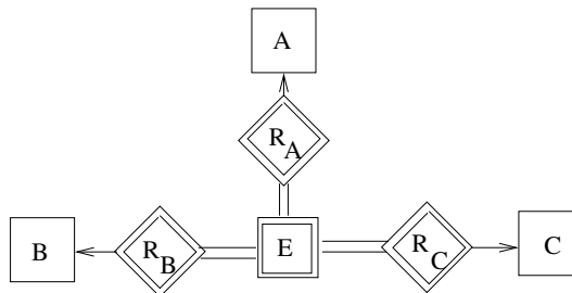
Figure 2.18 E-R diagram to Exercise 2.17d.
